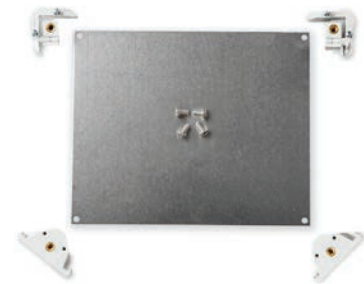
Hinged Front Panel Kit
